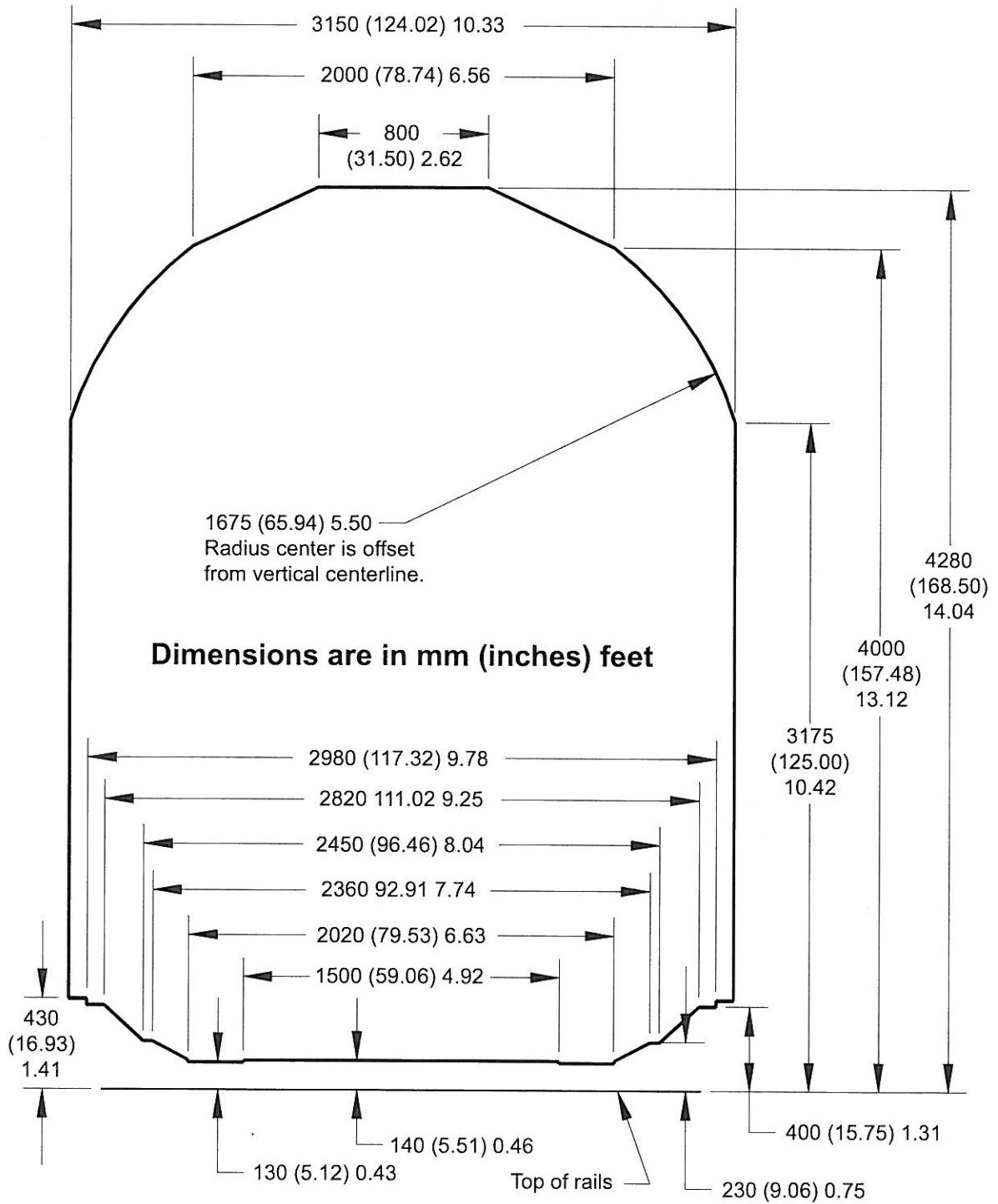
Figure 6. GIC Diagram.
