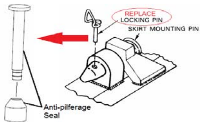
Mounting Pins (seal replaces locking pin)
