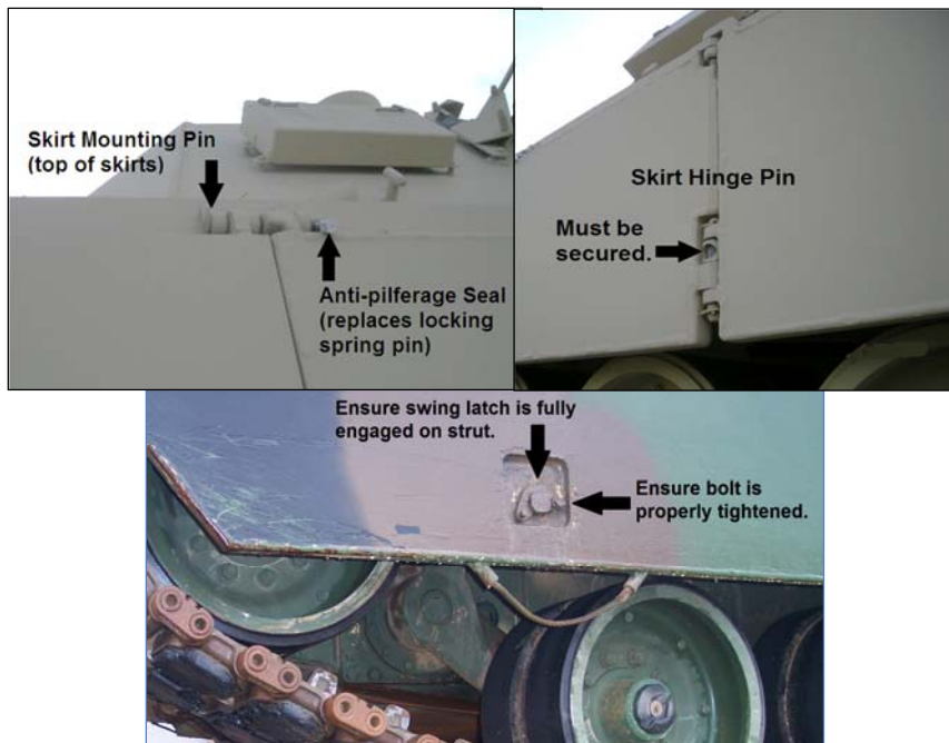
Mounting Pins (seal replaces locking pin)
